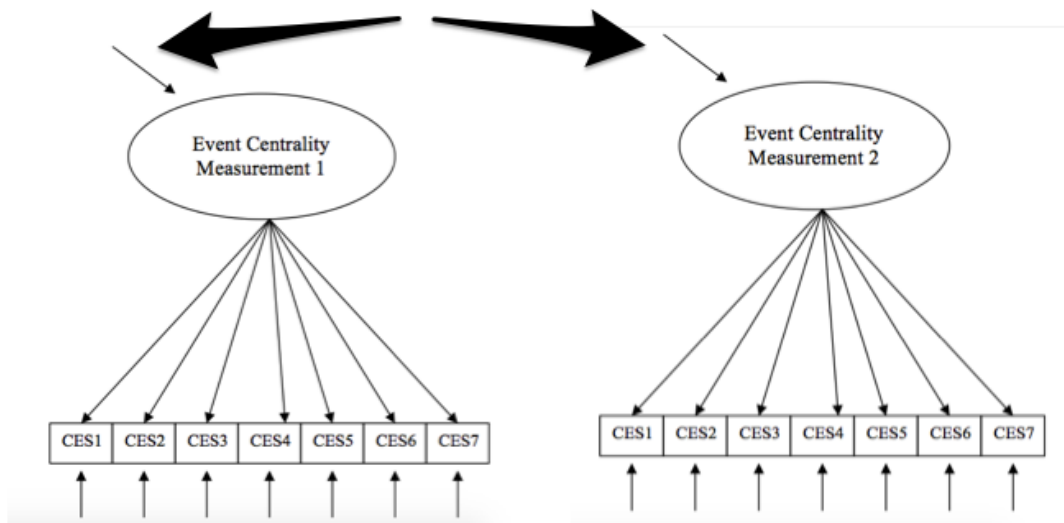
Model 6: All prior constraints plus latent variable residuals (i.e., variances of the overall scale) are similar.
